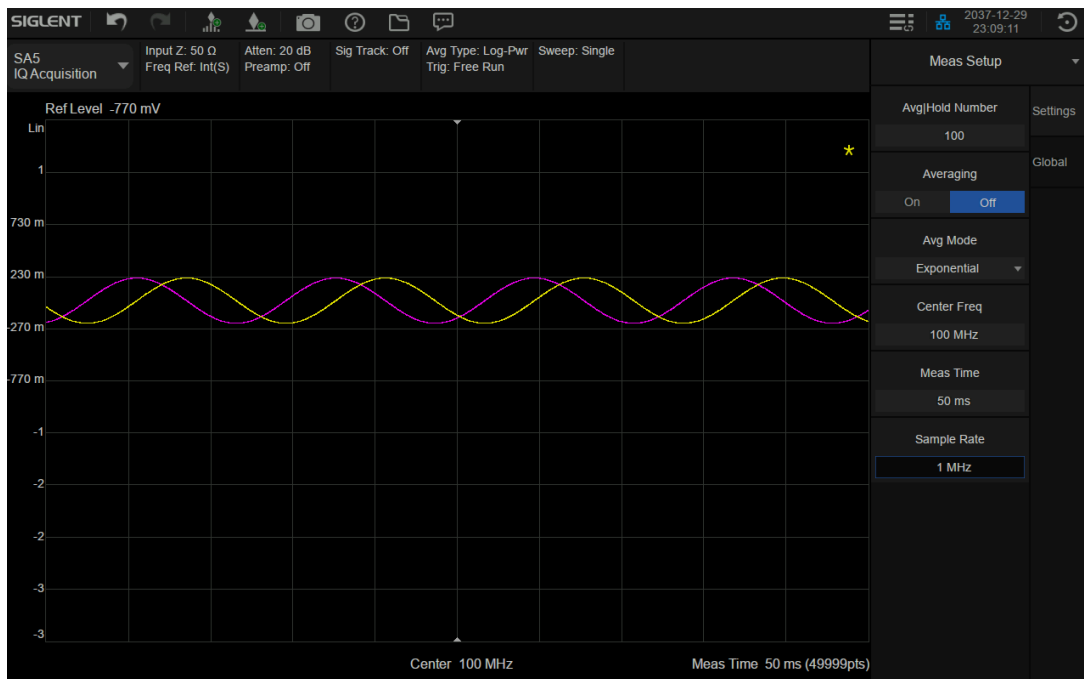
Figure 3-16 IQ Acquisition
