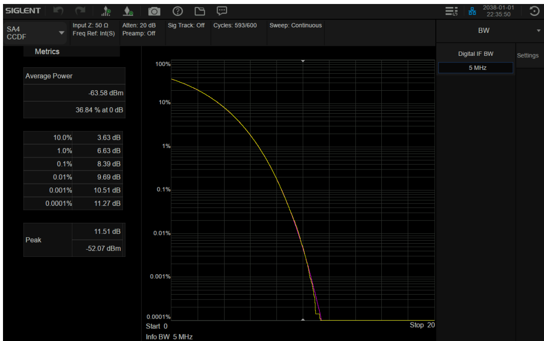
Figure 3-17 CCDF
